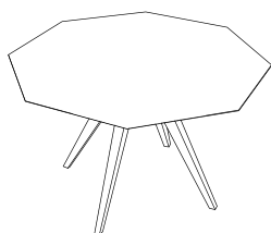
OTE937 DADO OCTAGONAL WOODEN TOP TABLE H=77 W=120 D=120 seats up to 6 people
